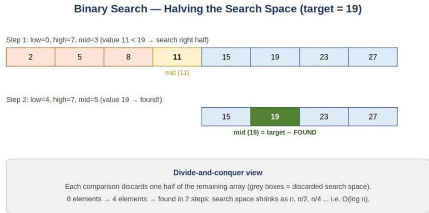
Fig. 3 — Binary Search narrowing the search range by half at each comparison.
